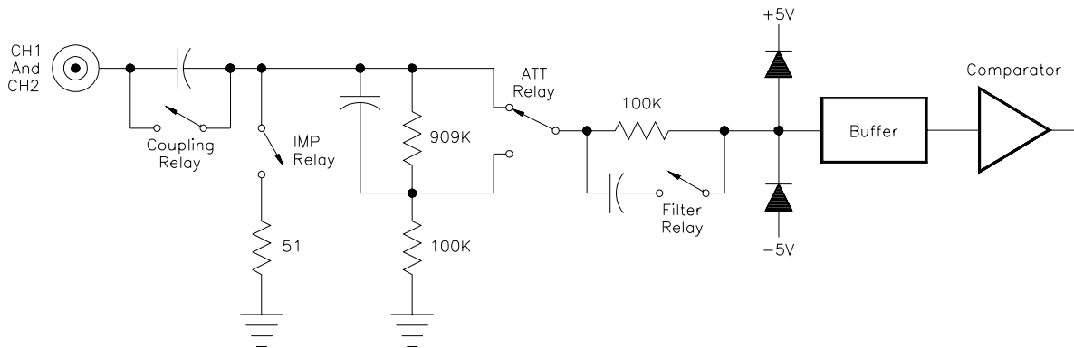
Figure 1-1. Universal Counter Block Diagram
