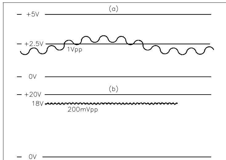
Figure 3-2. Using AC Coupling
