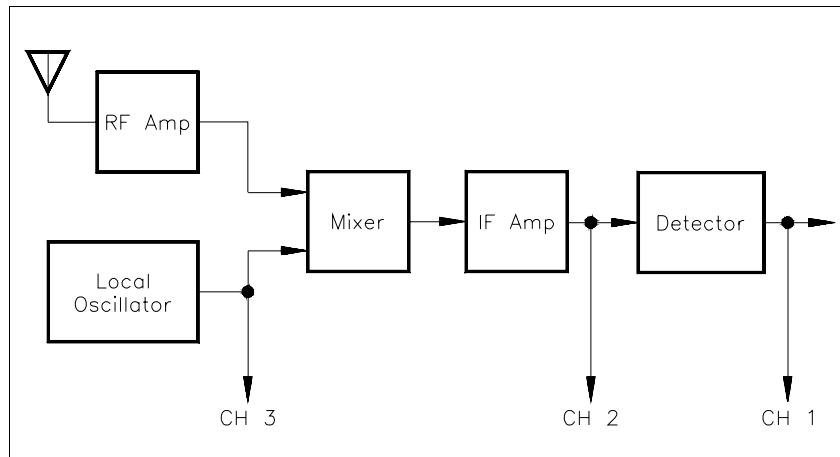
Figure 3-4. Frequency Measurement
